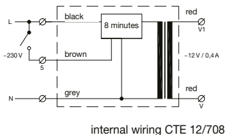
internal wiring CTE 12/708
