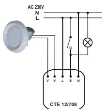
wiring CTE 12/708 with KEL
