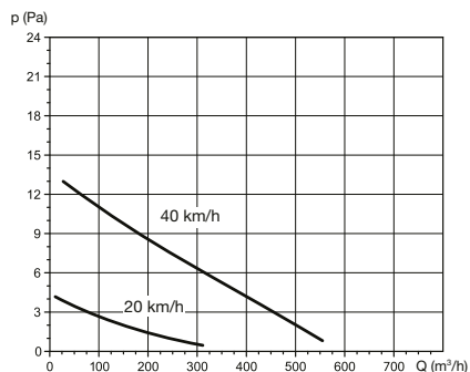
Pressure characteristics of the VH 315 roof head as a function of wind speed (indicative values)
