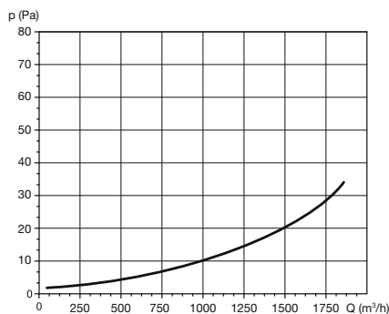
Roof head pressure loss values VH 315 as a function of air flow in the discharge pipe (indicative values)
