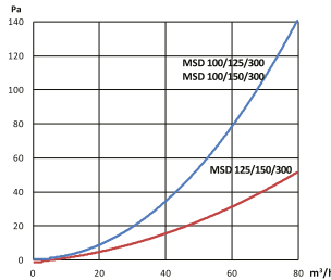
pressure loss
