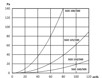
pressure loss
