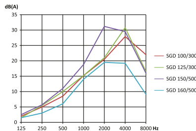
insertion attenuation
