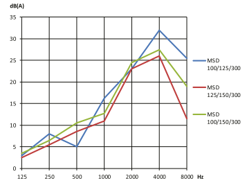
insertion attenuation
