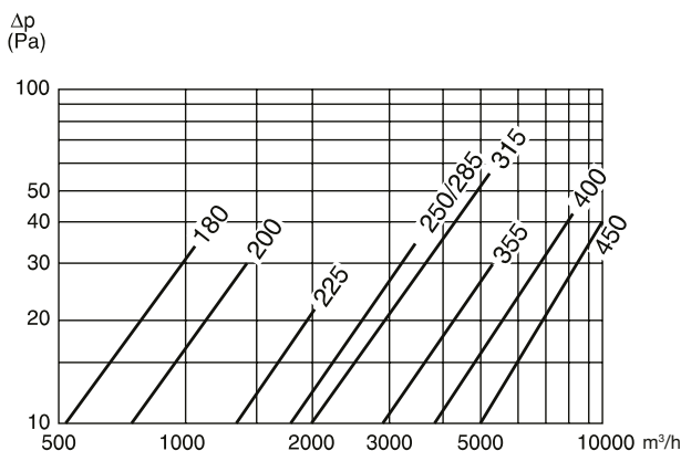
pressure losses depending on the flow rate
